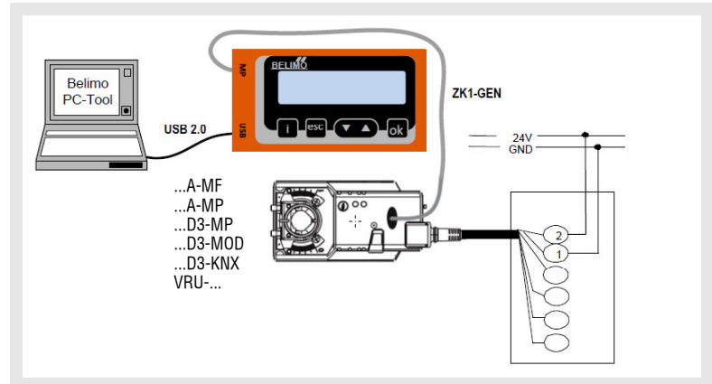
Connection diagram 1
