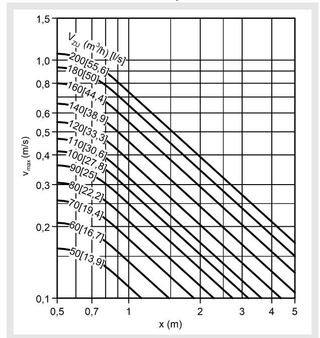
PILB-E-2-...-1000-150, two-way throw
