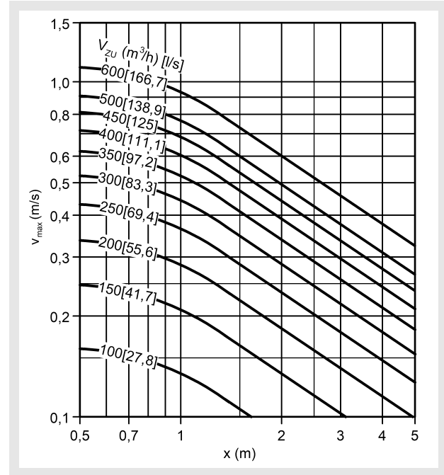
PILB-Q-2-...-0500-500, two-way throw
