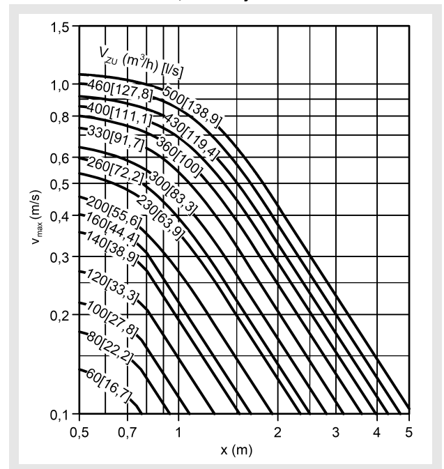
PILB-E-2-...-1000-300, two-way throw
