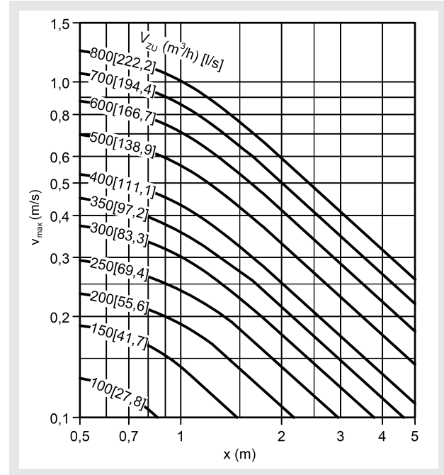
PILB-Q-2-...-0600-600, two-way throw
