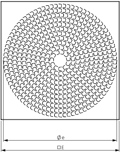
Diffuser shape Q
