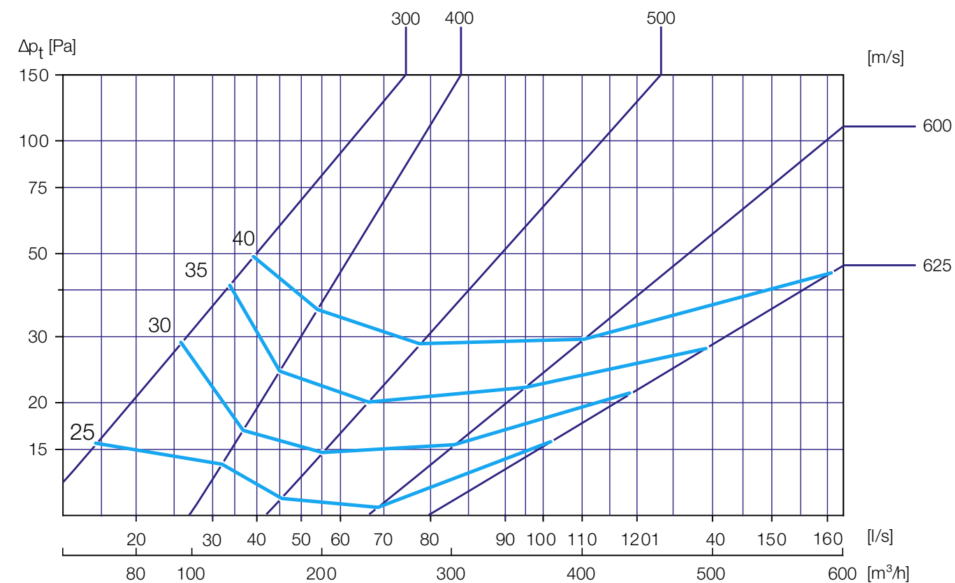
Quick selection DOR-Q-PBQ
